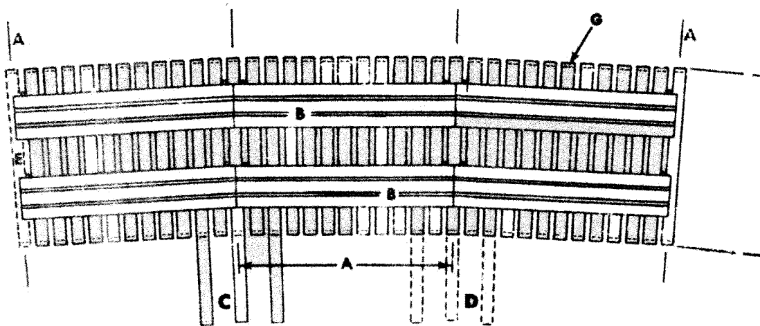
32" RADIUS
